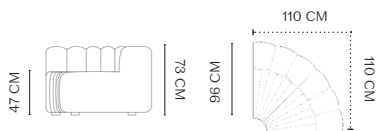
STUDIO CORNER W 110 CM / D 96 CM / H 73 CM SH 47 CM / SD 61 CM
